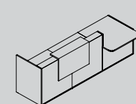
TRA39L 3056 / 1120 / 1159 120 3/8" / 44 1/8" / 45 5/8" TRA39P 3056 / 1120 / 1159 120 3/8" / 44 1/8" / 45 5/8" TRA40L 3456 / 1120 / 1159 136 1/8" / 44 1/8" / 45 5/8" TRA40P 3456 / 1120 / 1159 136 1/8" / 44 1/8" / 45 5/8" TRA41L 3856 / 1120 / 1159 151 3/4" / 44 1/8" / 45 5/8" TRA41P 3856 / 1120 / 1159 151 3/4" / 44 1/8" / 45 5/8"
