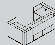
TRA29 3240 / 1705 / 1159 127 1/2" / 67 1/8" / 45 5/8" TRA30 3640 / 1705 / 1159 143 1/4" / 67 1/8" / 45 5/8" TRA31 4040 / 1705 / 1159 159" / 67 1/8" / 45 5/8" TRA32 4440 / 1705 / 1159 174 3/4" / 67 1/8" / 45 5/8"
